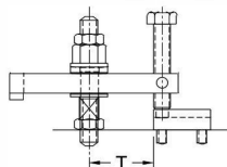
Hex-Head Clamping Screw CL-xx-THPA-HH
