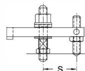
Oval-Point Clamp Rest CL-xx-THPA-OP
