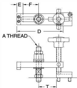
Hand-Knob Clamping Screw CL-xx-THPA-HK
